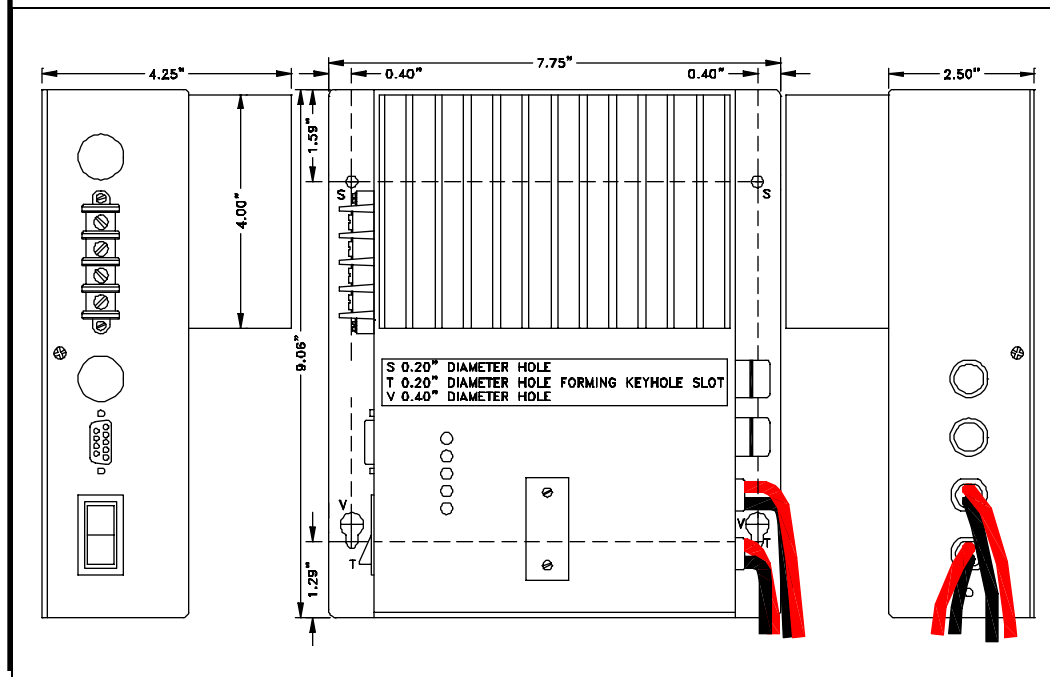
Mechanical Diagram
