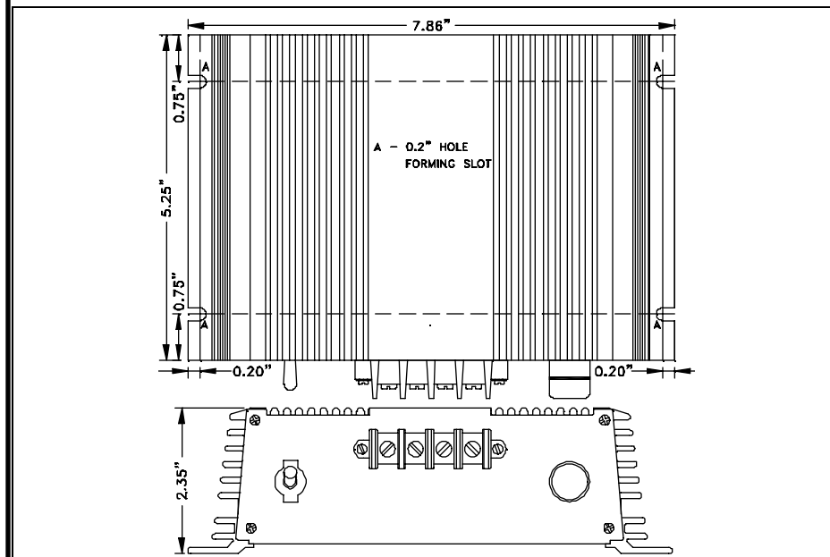
Mechanical Diagram
