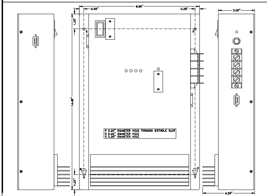
Mechanical Diagram
