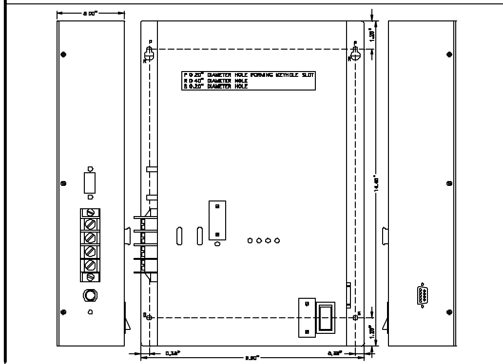
Mechanical Diagram
