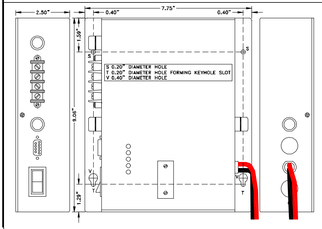
Mechanical Diagram
